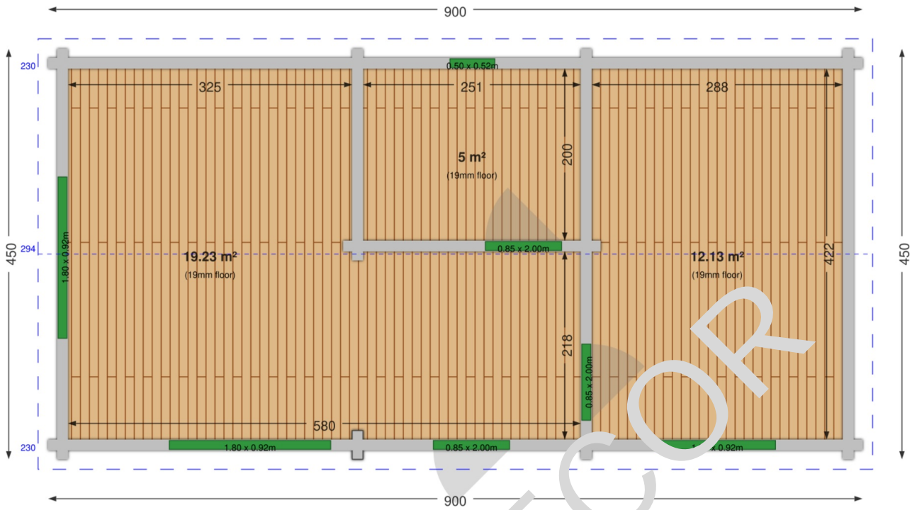
Top view
