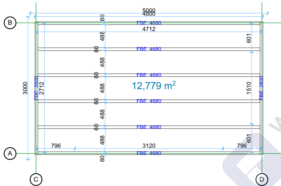
Floor bearers 1:50
