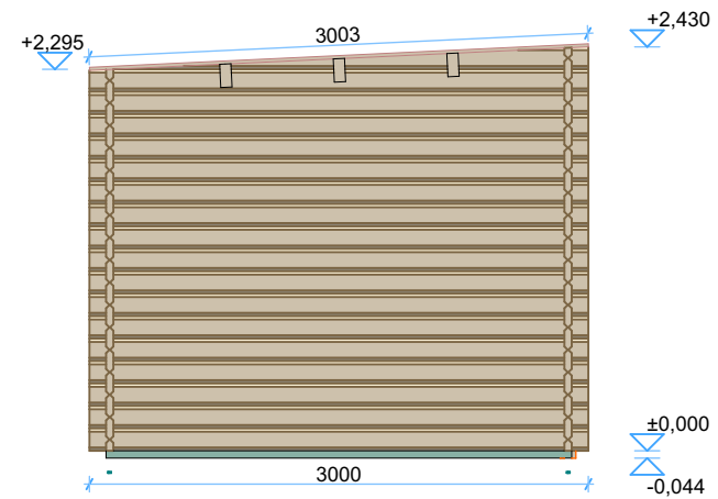
Left Elevation
