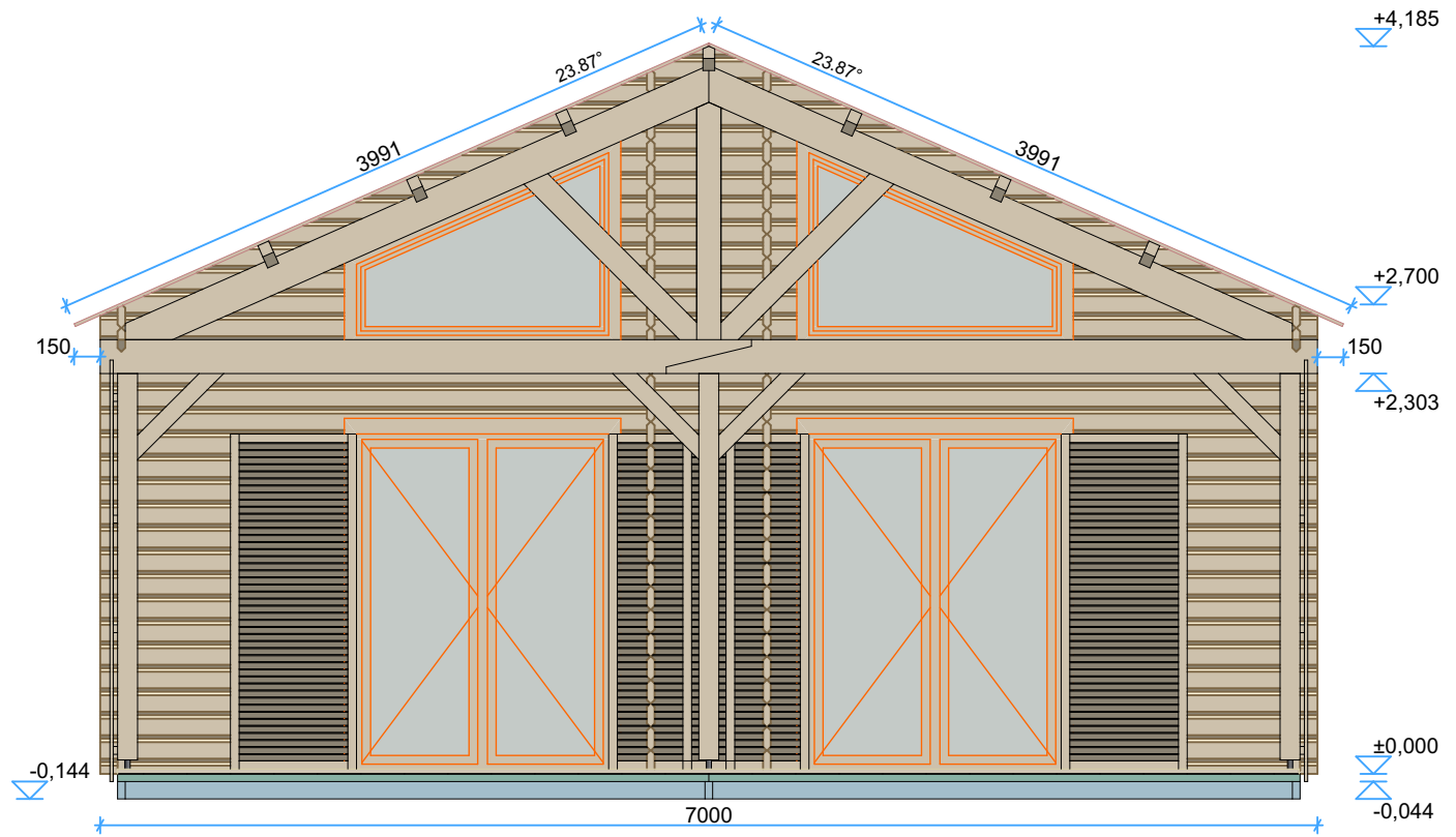
Front Elevation
